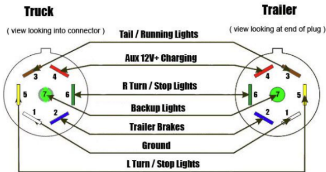
7-way RV Style Trailer Plug Wiring (aka Pollock or Bargman plug)
